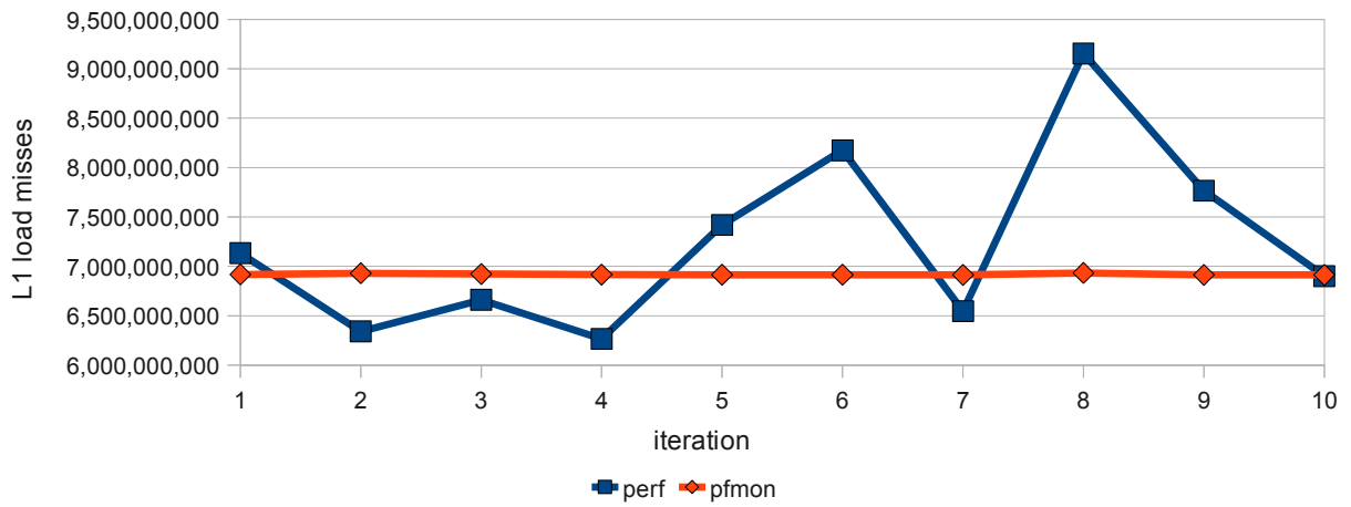
L1 load misses on POWER6
