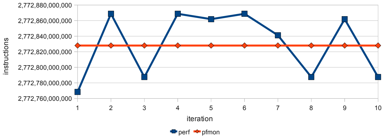
instructions completed on POWER6
